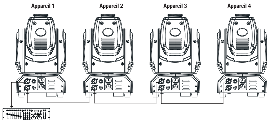
Console DMX
